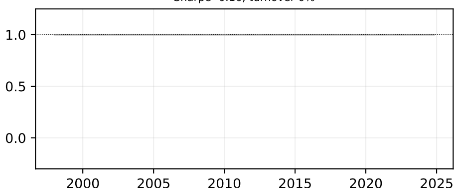
Turnover penalty 1 Sharpe -0.16; turnover 0%
