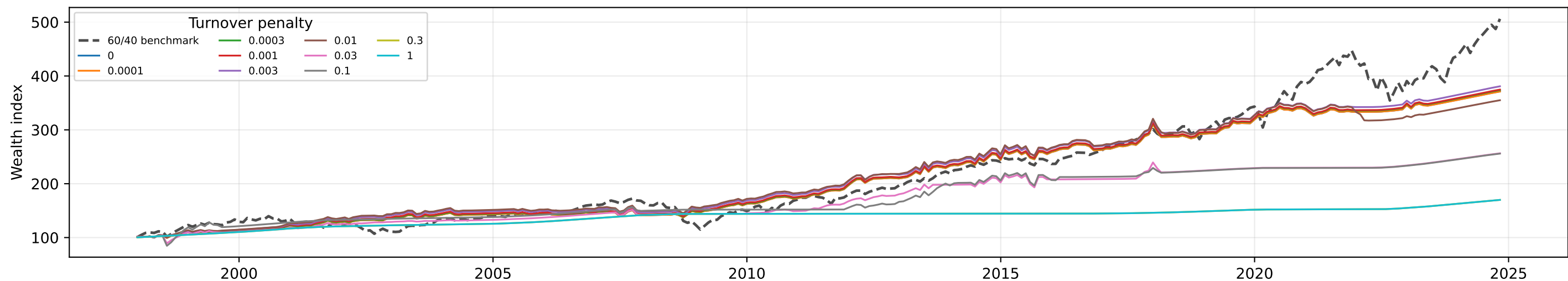
Turnover penalty 0 Sharpe 0.55; turnover 170%
