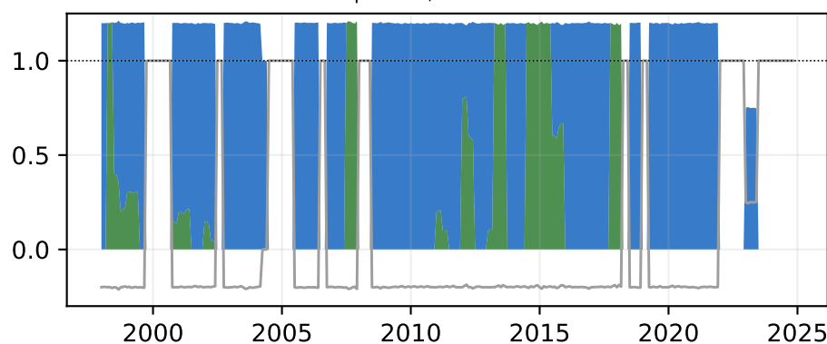
Turnover penalty 0.003 Sharpe 0.58; turnover 167%
