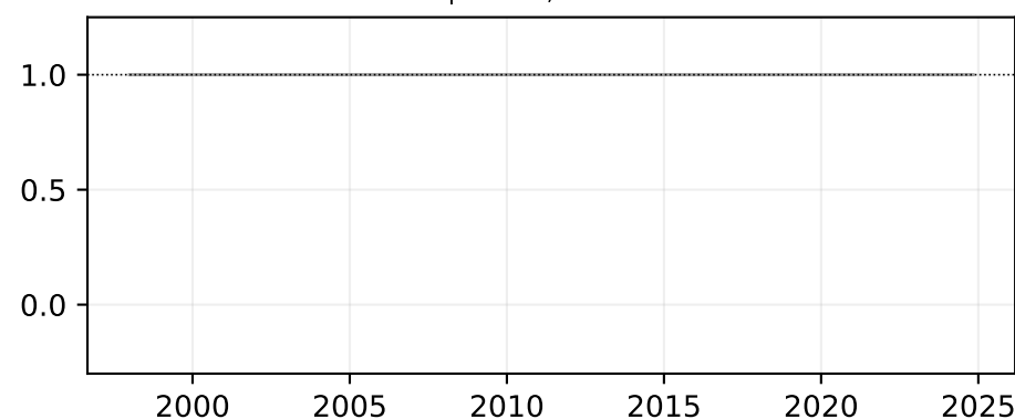
Turnover penalty 0.3 Sharpe -0.16; turnover 0%
