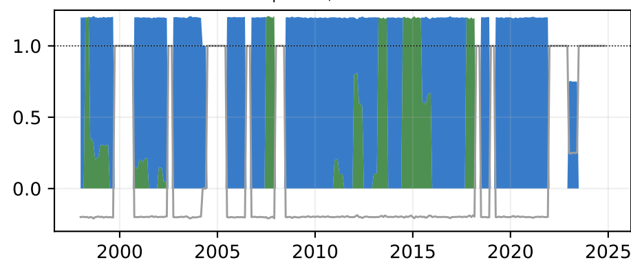
Turnover penalty 0.01 Sharpe 0.51; turnover 156%
