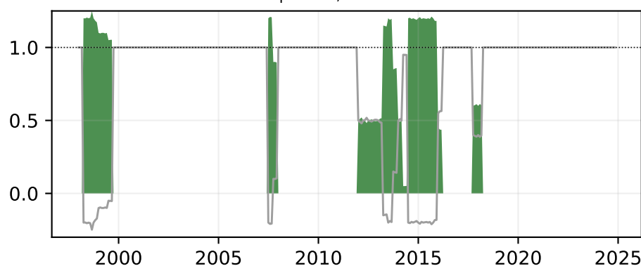
Turnover penalty 0.1 Sharpe 0.26; turnover 40%
