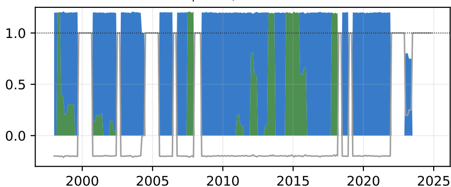
Turnover penalty 0.001 Sharpe 0.56; turnover 168%
